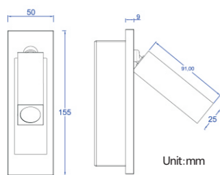
Cutout size: L130 x W40 x H42mm
