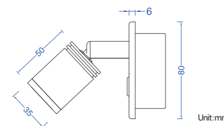
Cutout size: D50 x H50mm
