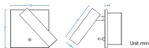
Cutout size: L95 x W55 x H45mm
