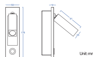
Cutout size: L160 x W40 x H60mm
